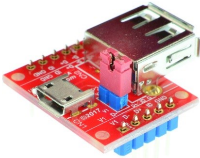
Figure 3: USB-uBF-AF-V1A with headers
