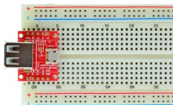
Figure 2: Example of connecting the USB-uBF-AF-V1A on a breadboard (Note: This picture only shows the pins spacing, actual use may not be used on a breadboard)
